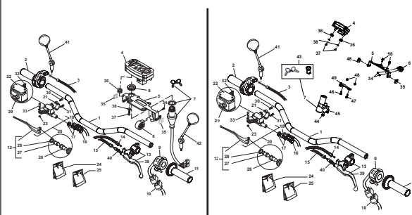
TAV.35 Manubrio - Handlebars - Guidon - Lenker - Manillar
