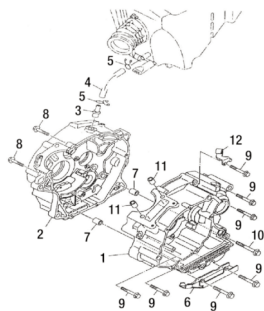
TAV.01A Carter motore - Crankcase assy. - Carter moteur complet - Kurbelgehäuse, compl. - Carter motor completo
