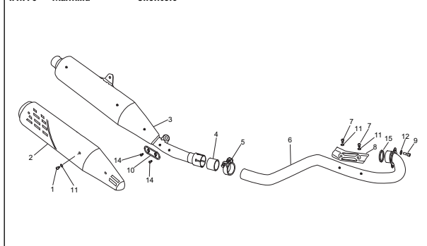
TAV.10 - Marmitta - Silencers
