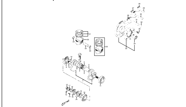
TAV.4 - Albero motore-pistone - Crankshaft-Piston
