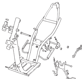
TAV.15 Telaio-Cavalletto - Chassis-Central stand - Châssis-Bequille - Rahmen-Ständer - Chasis-Caballote
