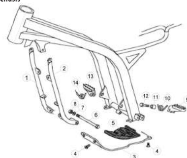
TAV.32 Accessori telaio - Frame accessories - Accessoires chassis - Rahmenzubehö ren - Accesorios Chasis
