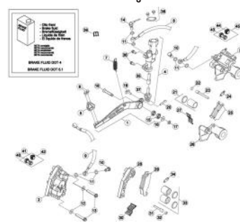
TAV.36 Impianto freni idraulici - Hydraulic brakes system - Installation des freins hydrauliques - Hydraulischebremse anlage - instalaci3n freno hidr3ulico
