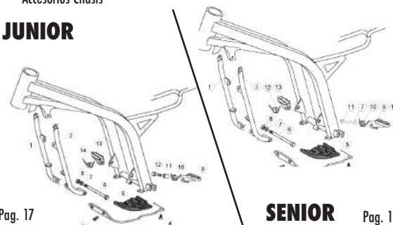
TAV.32 Accessori telaio - Frame accessories - Accessoires chassis - Rahmenzubehö ren - Accesorios Chasis
